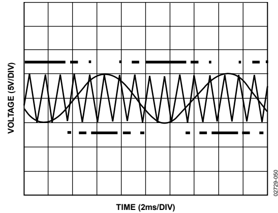
Figure 56. Pulse-Width Modulation
