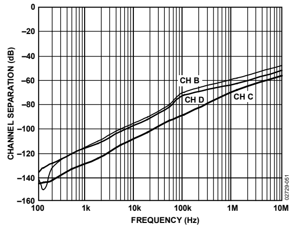
Figure 57. Channel Separation
